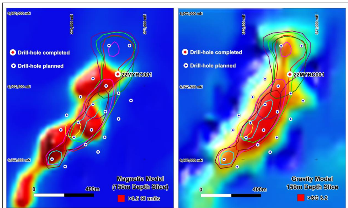
Figure 1 shows the planned drill-holes with respect to both the magnetic and gravity models. The areas shown in red are both strongly magnetic (magnetic susceptibility >0.5 SI units) and have high density (average SGs >3.2), outlining the potential magnetite (Fe) target.
